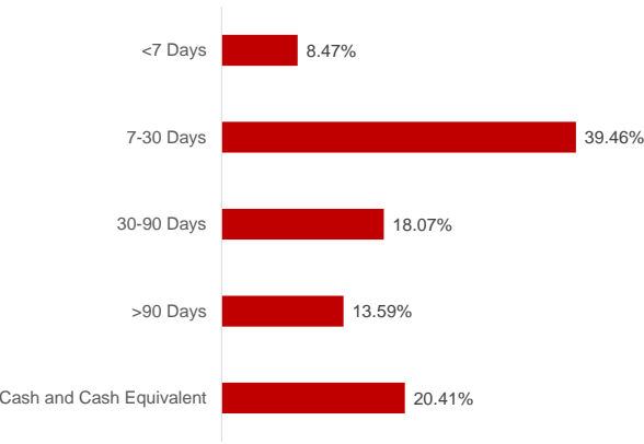
Maturity Allocation (%)
